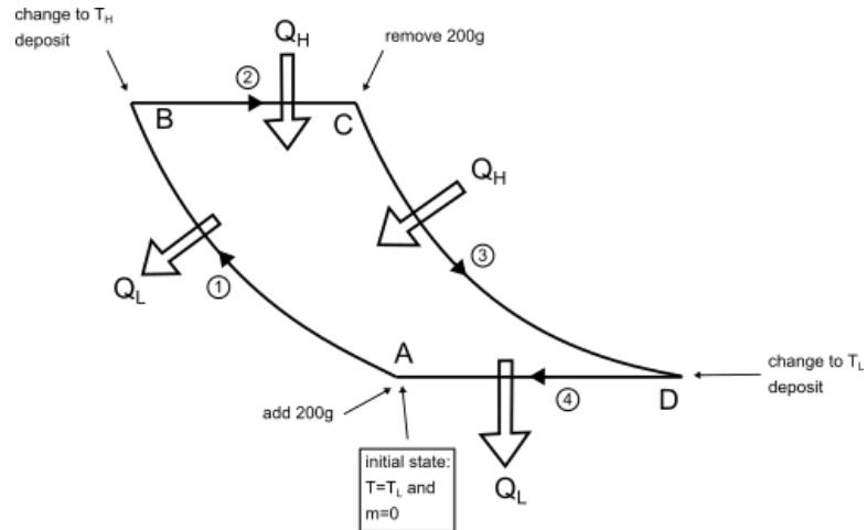
Figure 2: Heat and work in all processes
