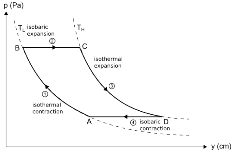
Figure 1: Our thermodynamic cycle
